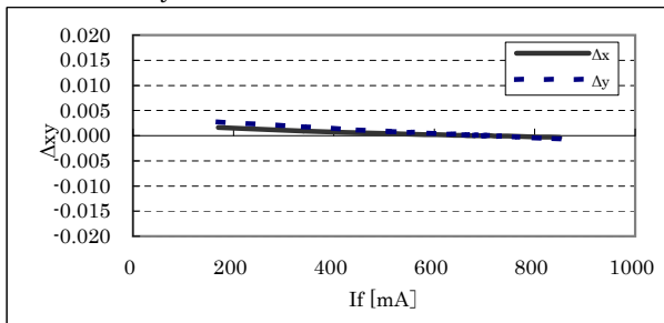
5-3 If- \Delta_{xy} characteristics (If=350mA)
