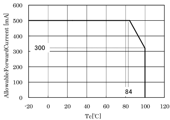
◆ Case Temperature vs. Allowable Forward Current
