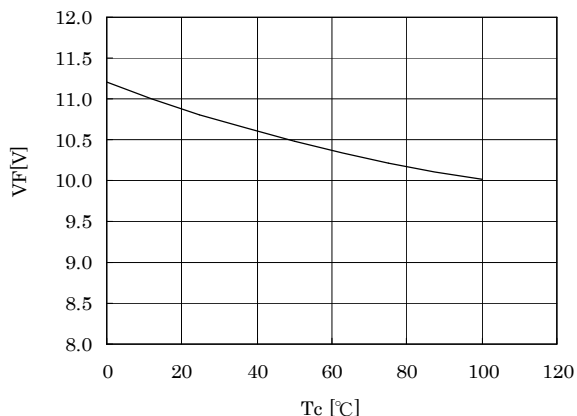
◆ Case Temperature vs. Forward Voltage
