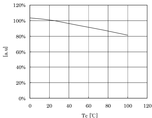
◆ Case Temperature vs. Relative Luminous Flux
