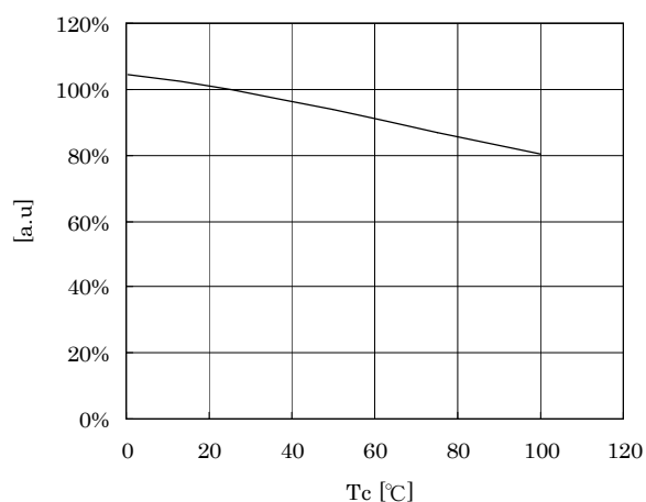
◆ Case Temperature vs. Relative Luminous Flux
