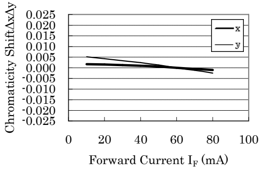
I_F - \Delta x \Delta y Characteristic T_C = 25^\circ C
