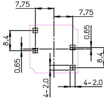
PAD position layout
