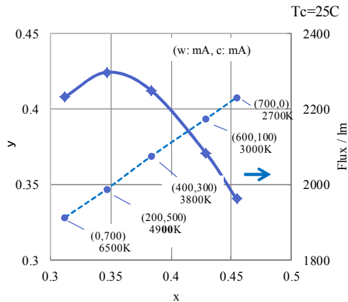
xy shifting curve & flux curve
