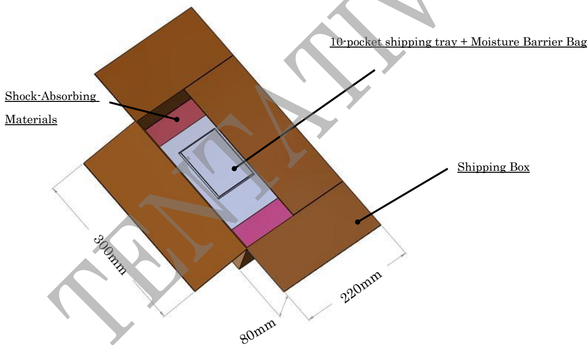
Packaging of Shipping Trays (2 trays max.)
