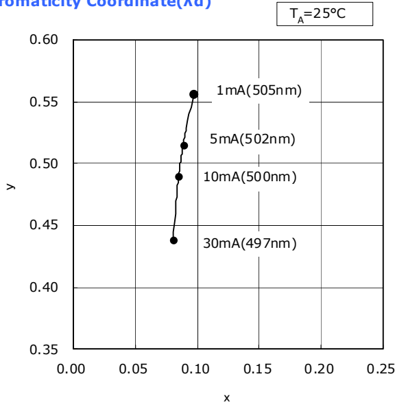
順電流-色度(主波長)特性 Forward Current vs Chromaticity Coordinate( \lambda_d )
